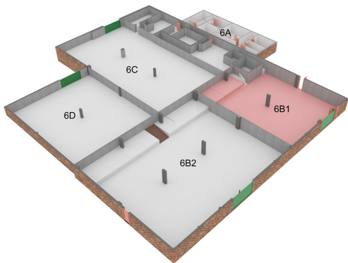
Building #6, Unit 6B1 plan
